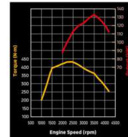
2.4-litre MIVEC Turbocharged DOHC DI-D High power (133kW/3500rpm, 430N·m/2500rpm)
